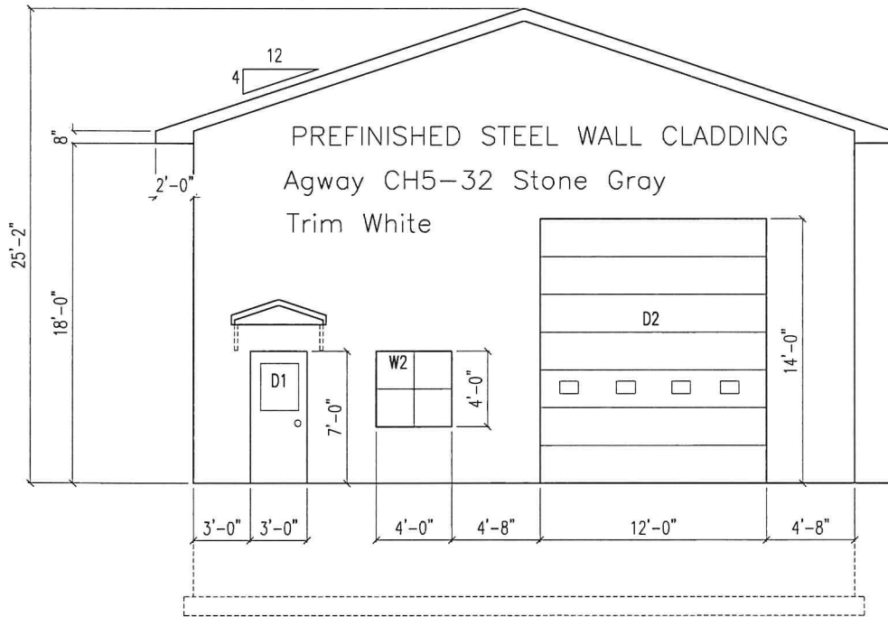
FRONT ELEVATION SCALE 1=48
