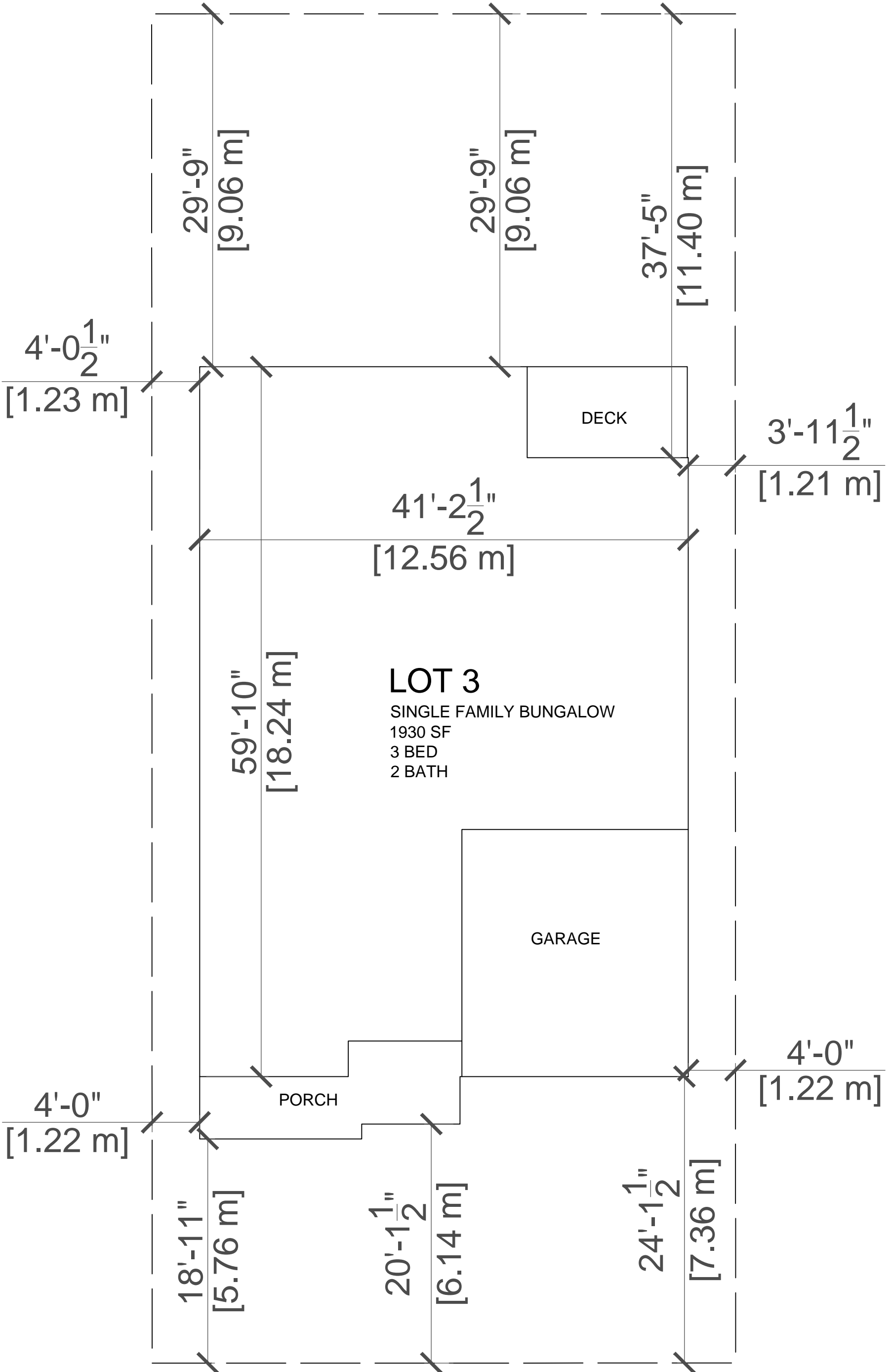
LOT 3 WEST MEADOWS SITE PLAN
