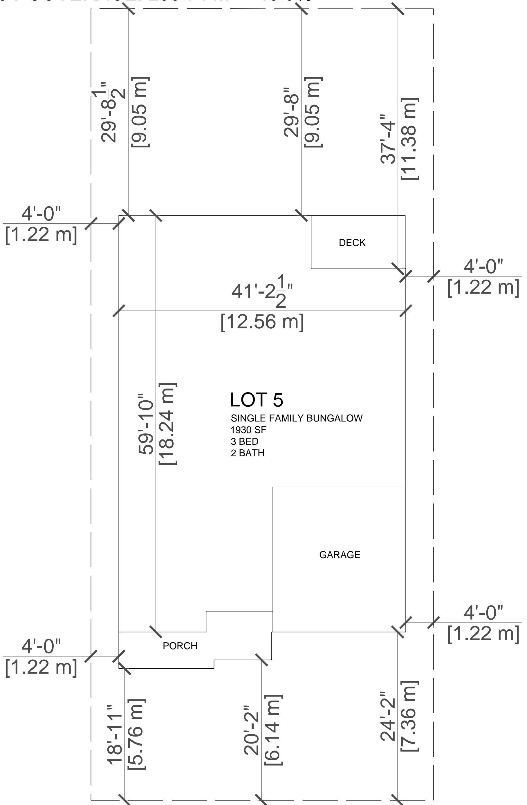
LOT 5 WEST MEADOWS SITE PLAN
