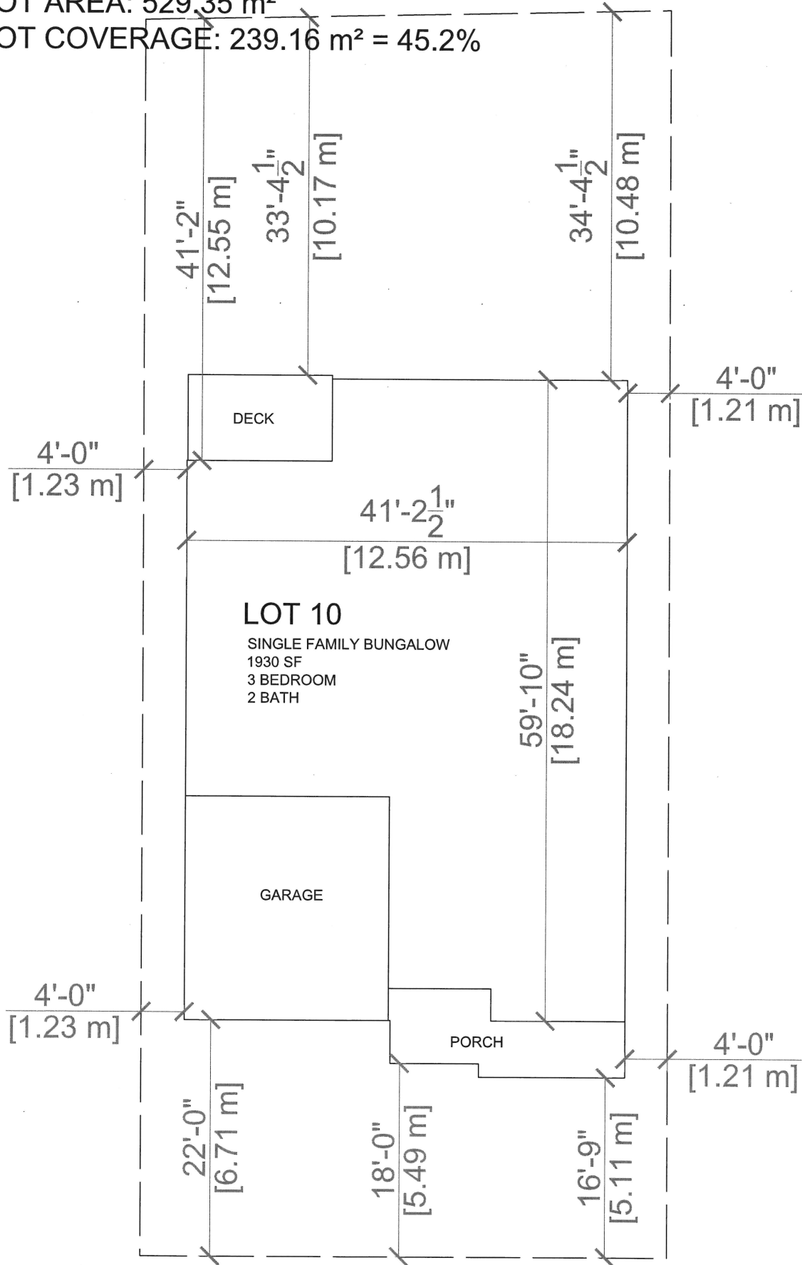
LOT 10 WEST MEADOWS SITE PLAN
