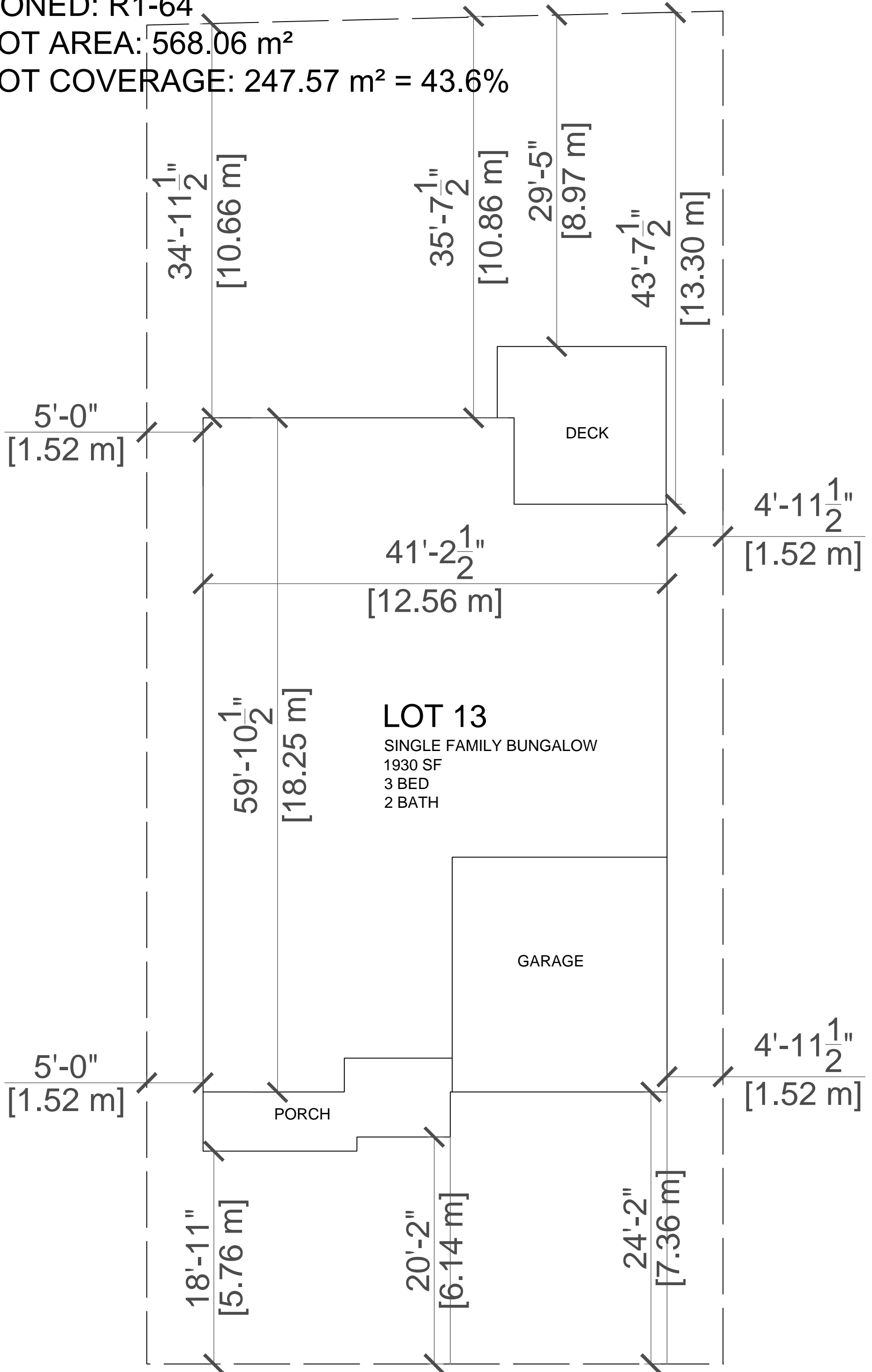
LOT 13 WEST MEADOWS SITE PLAN
