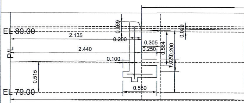
1 FRONT YARD X-SECTION - NORTH SE4 1:25
