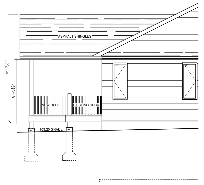
2 SIDE ELEVATION A-
