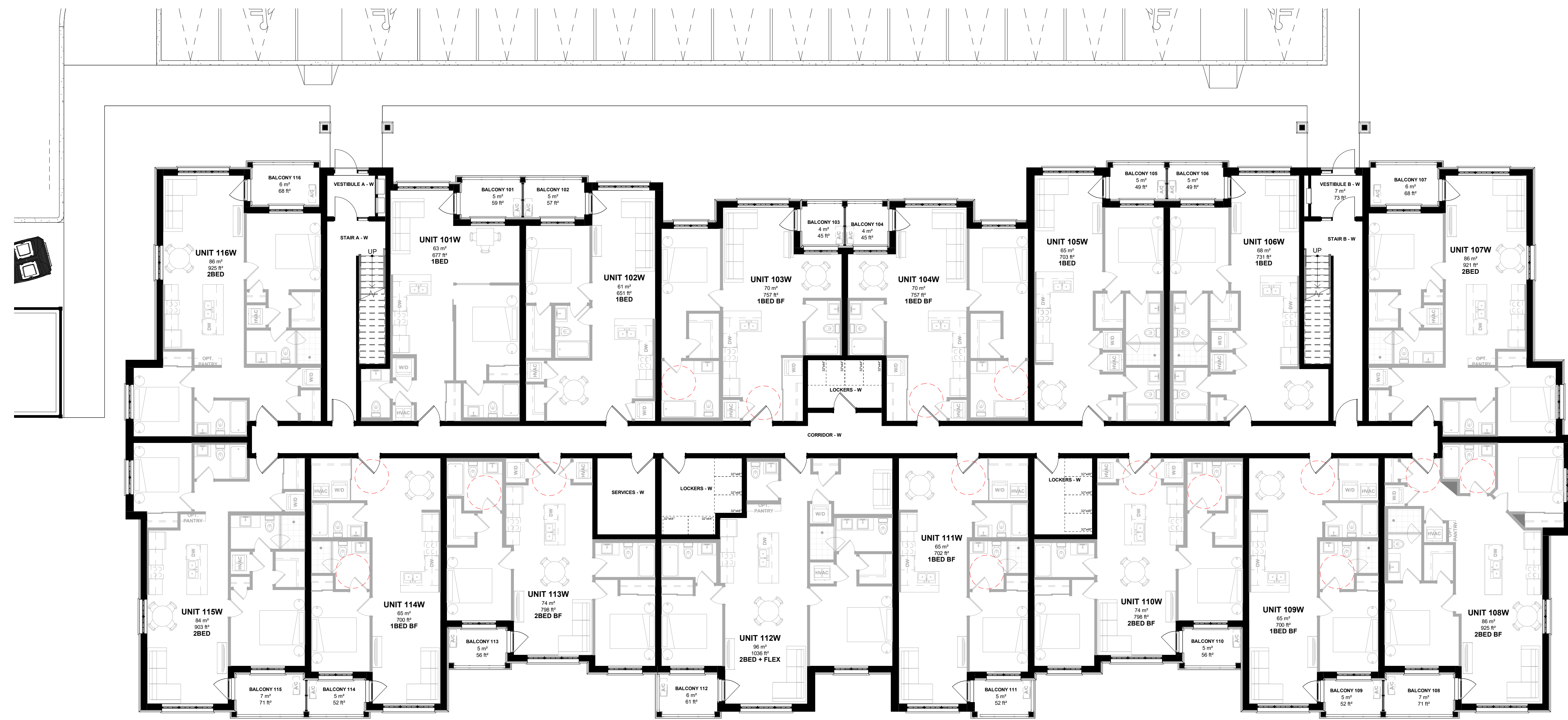
2 WEST BUILDING - GROUND FLOOR SK.01 1:100
