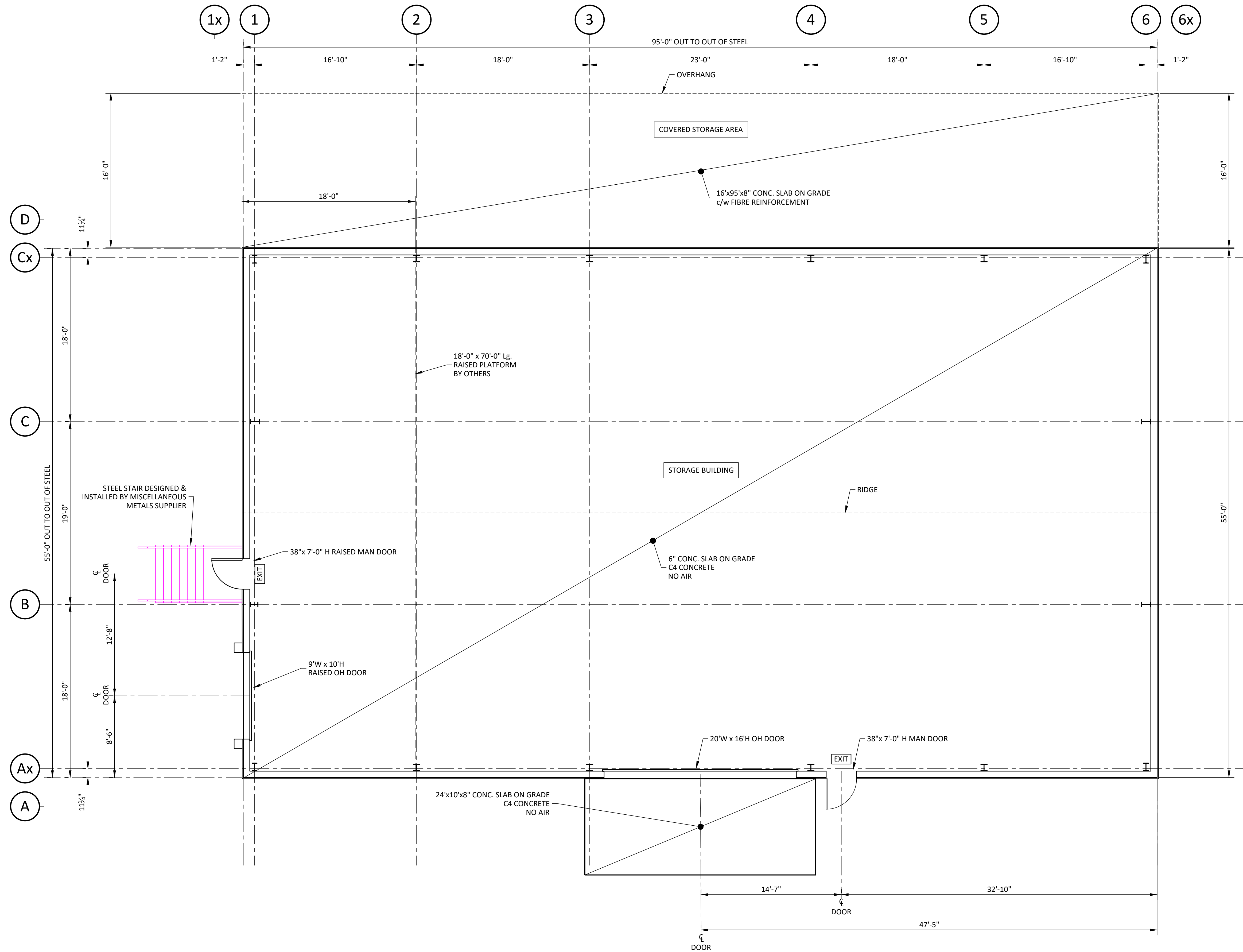
1 FLOOR PLAN A-1 3/16"=1'-0"
