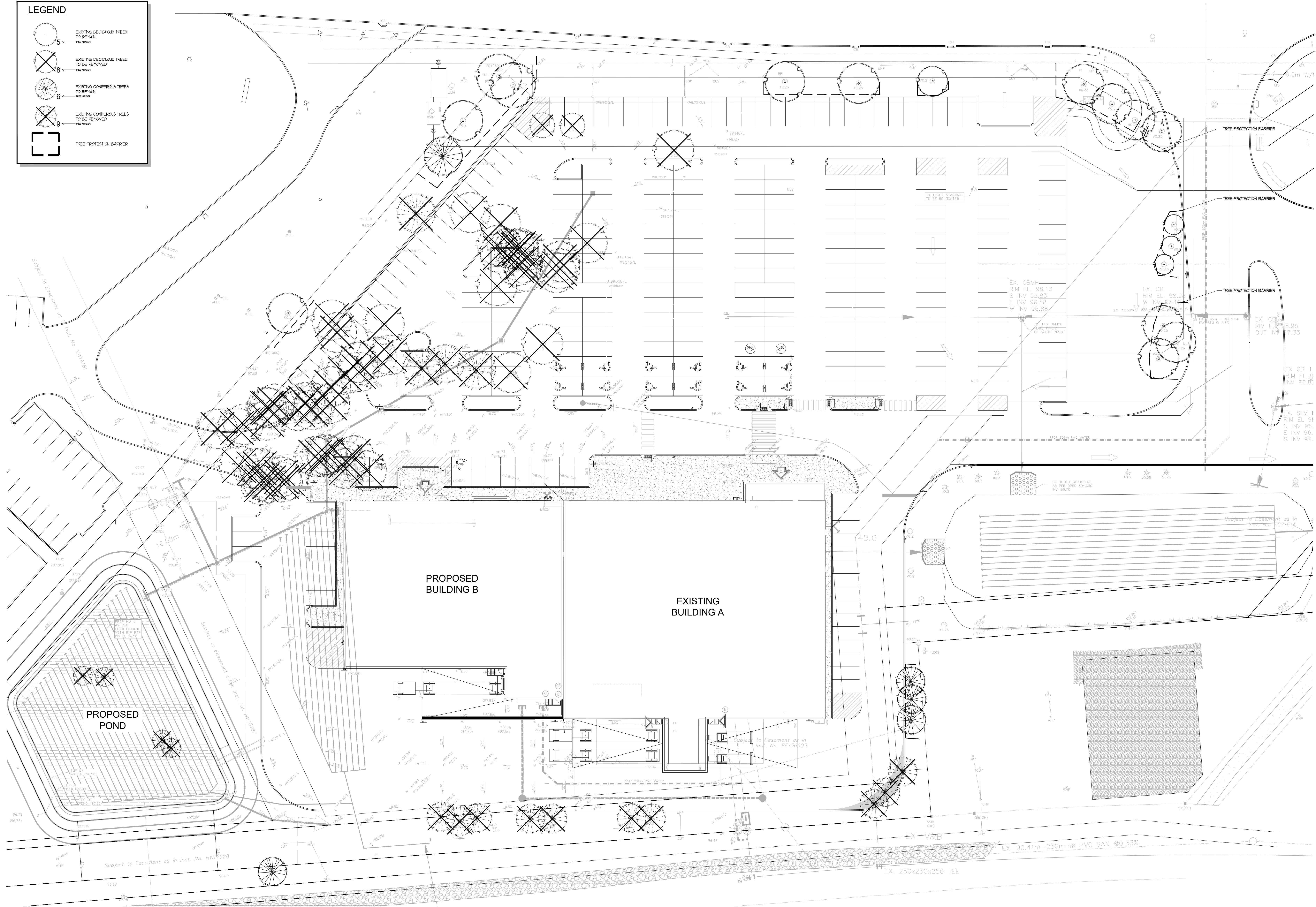
TREE PRESERVATION PLAN SCALE = 1:300
